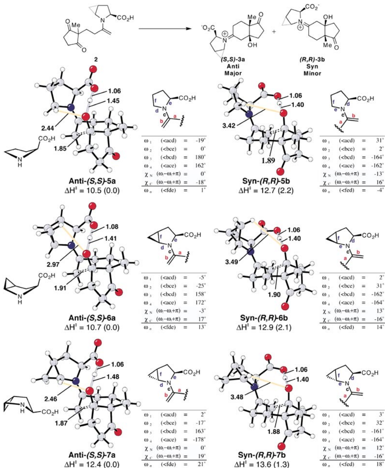
Figure 1. anti and syn transition structures for proline, cis - and trans -4,5-methanoproline catalyzed cyclization of enamine 2 (Hajos–Parrish–Eder–Sauer–Wiechert reaction). Shown on the tables are dihedral angles relevant to the measure of iminium planarity.
