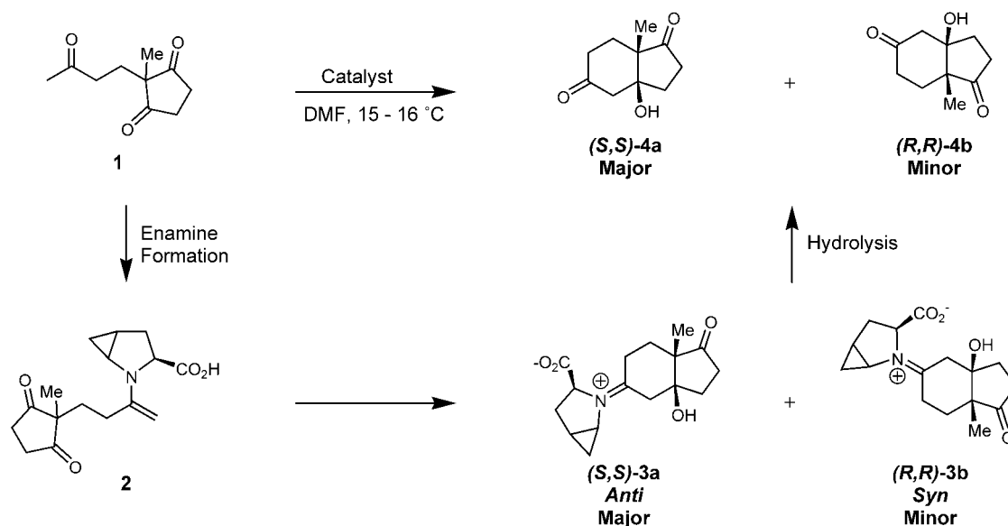
Scheme 1. Mechanism of proline derivative-catalyzed Hajos–Parrish–Eder–Sauer–Wiechert reaction.
